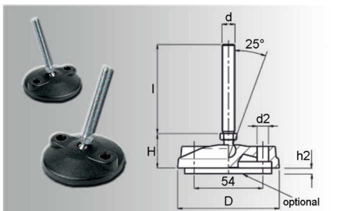
Adjustable feet with fixing holes
