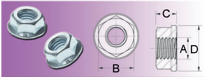
Hexagon nuts with flange - metal ~DIN 6923 without lock toothing (~DIN EN 1661)
